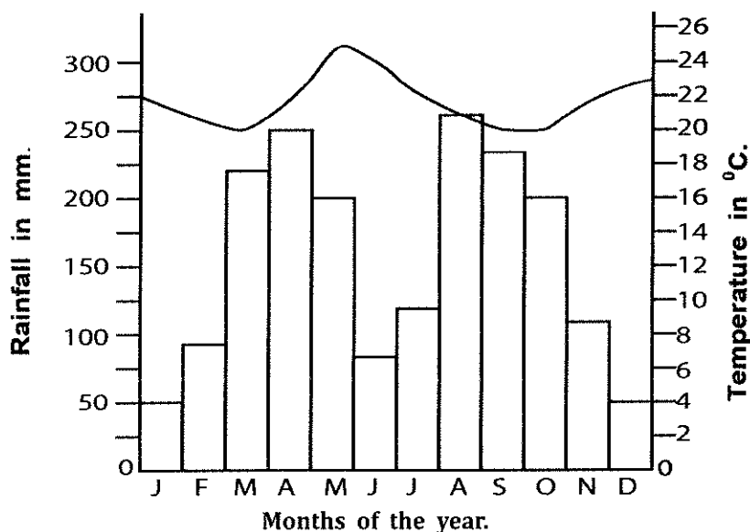
A graph showing equatorial climate
